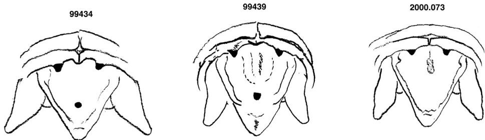
Fig. 22. Sketches of supra-anal plates of A.a.pulchra and A.a. annulicornis , showing differences in furcula and patterning. Specimens chosen to show range of form in both subspecies. The multidigit numbers are specimen numbers.
