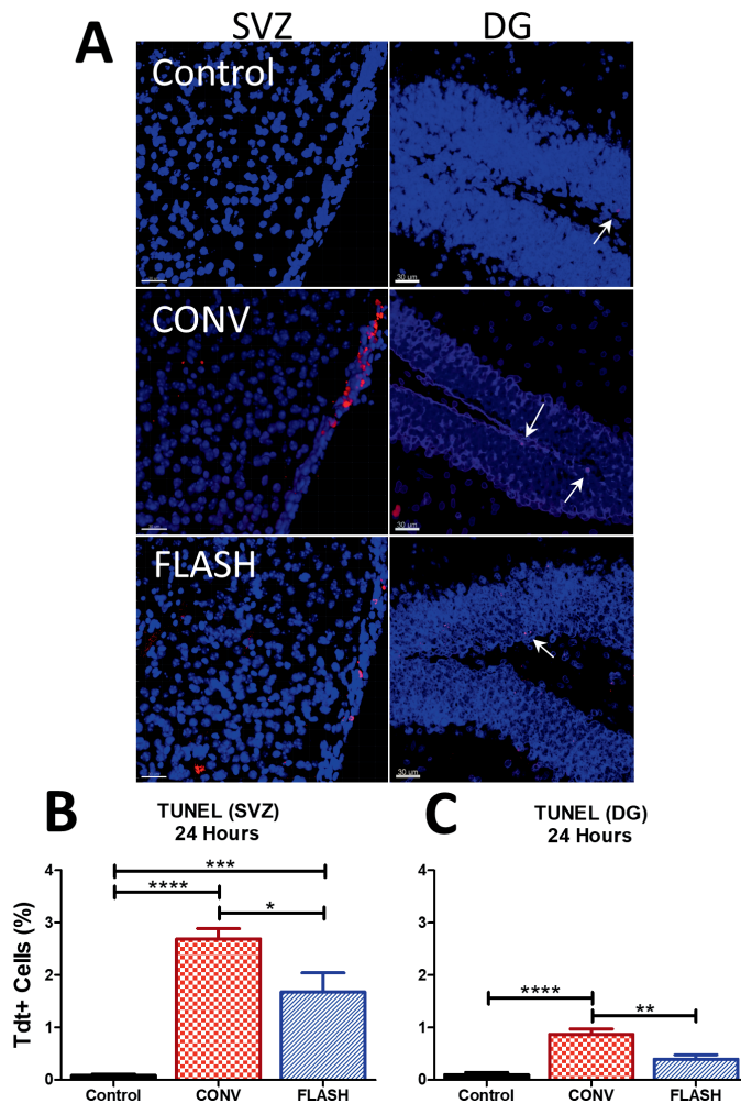
FIG. 4. FLASH reduces apoptosis compared to CONV within neurogenic regions, 24 h postirradiation. TUNEL assay was performed to determine levels of apoptosis within the dentate gyrus (DG) and subventricular zone (SVZ). CONV-irradiated animals exhibited a significant increase when compared to FLASH and control in both the SVZ and DG. Representative images of Tdt + cells within the SVZ (left side) and DG (right side). Scale bars = 30 \mu m). Panels B and C: Analysis of Tdt + cells within the SVZ and DG at 24 h postirradiation. Data is shown as the mean \pm SEM ( n = 6 per group, two images analyzed per animal). * P \leq 0.05 , ** P \leq 0.01 , *** P \leq 0.001 , **** P \leq 0.0001 (ANOVA with Bonferroni's multiple comparisons test).
