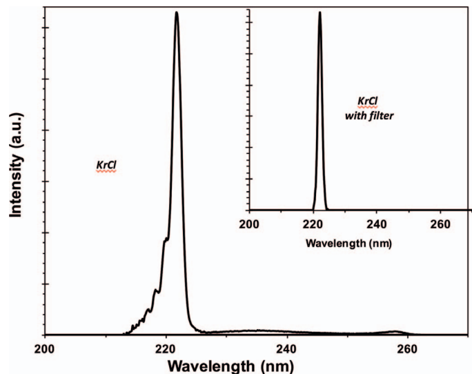
FIG. 1. Nonfiltered and filtered measured emission spectra from a Kr-Cl excimer lamp (main peak 222 nm).
