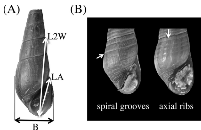
Fig. 1. (A) Morphometric characters used in present study. Abbreviations: B, shell width; L2W, height of first and second body whorls; LA, maximum dimension of the aperture. (B) Shell surface sculpture. Arrows point to spiral groove (left) or axial rib (right).
