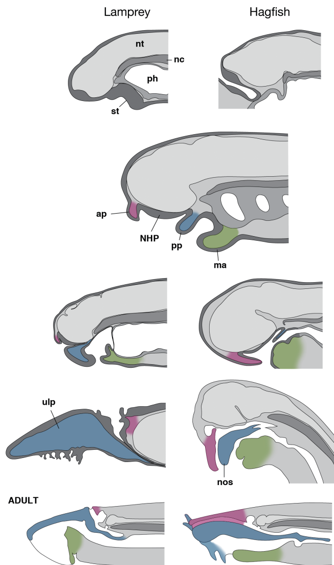
Fig. 1. Developmental pathways of lamprey and hagfish crania-facial patterns. The cyclostome pattern (second from the top) is schematically illustrated. This pattern appears after the establishment of the neural crest-derived ectomesenchyme.
