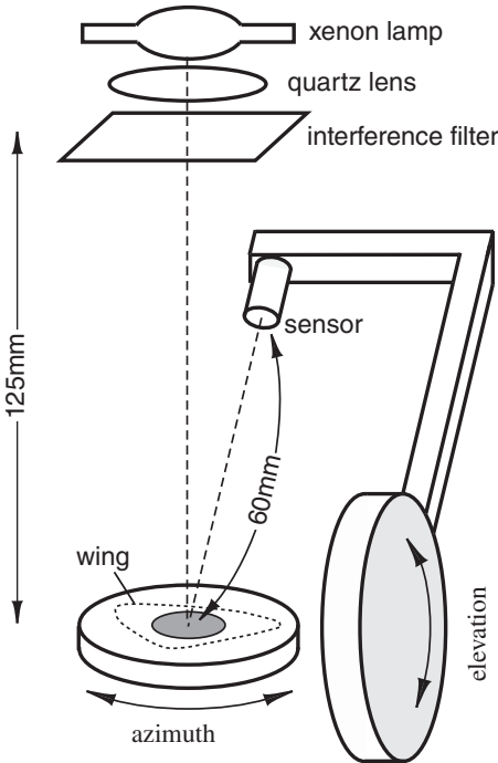
Fig. 4. Schematic of the device used for measurement of reflected light. Light passed through the interference filter is applied to the wing on the stage at the bottom. Reflected light from a circle of 8 mm in diameter is monitored by a sensor. Vertical shifting of the sensor and horizontal rotation of the stage provided hemispherical distribution data of reflected light.
