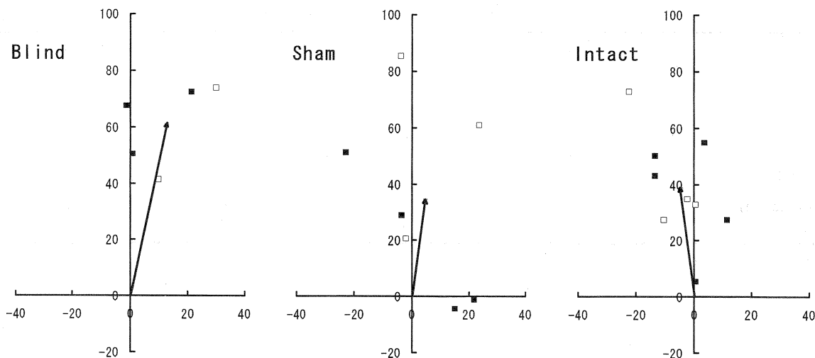
FIG. 5. Terminal points of vectors (small squares) representing migration of blind, sham-operated and intact toads captured at locations 50 to 100 m from the breeding pond, immediately operated and released soon after the operations. The initial point of each vector is taken at the origin of the axes, and the direction of the pond is 0 degree (the upward of the Y-axis). Empty and filled squares represent females and males, respectively. The mean vector is also indicated with an arrow. The unit of the axis values is m.
