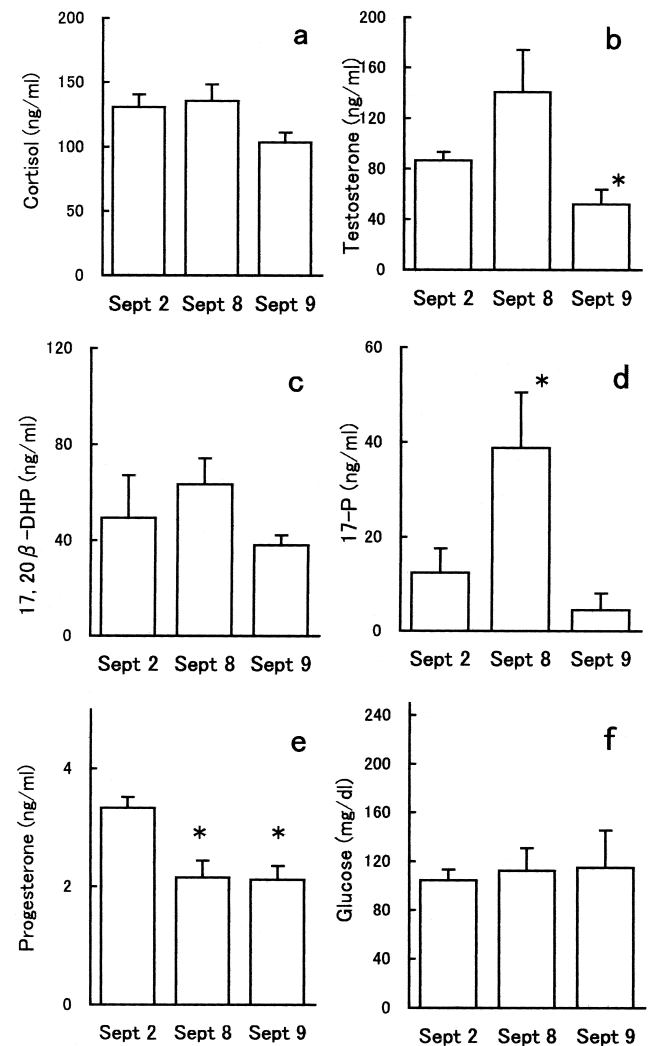
Fig. 5. Changes in mean plasma cortisol (a), testosterone (b), 17,20 \beta -dihydroxy-4-pregnen-3-one (17,20 \beta -DHP) (c), 17-hydroxyprogesterone (17-P) (d), progesterone (e) and glucose (f) levels in unhandled female sockeye salmon on one day and one week before stress experiment. Results on 9 September correspond to values of time zero at the experiment. *Significantly different at P \leq 0.01 when compared with hormone levels on 2 September. The number of fish was 10, 10 and 5 on 2, 8 and 9 September, respectively.
