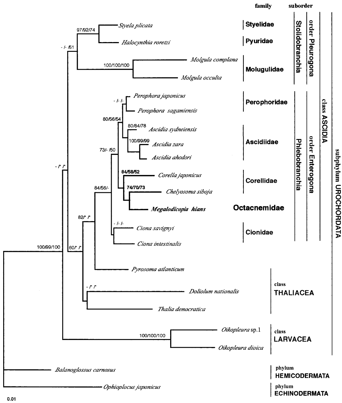
Fig. 1. Ascidian phylogeny estimated from 821 nucleotide sites of 18S rDNA. The NJ tree reconstructed by using the Kimura two-parameter distance is shown here. The numbers on each branch indicate BP values in the NJ/MP/ML trees. The values were calculated based on 1,000 resamplings in the case of NJ and MP and by 100 in the case of ML. Minus marks (–) denote < 50% bp values. Asterisks (*) indicate the nodes that did not appear in each MP and ML tree, or unresolved nodes in the majority consensus tree of 12 MP trees.
