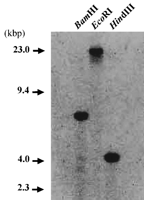
Fig. 6. Genomic Southern hybridization analysis. Genomic DNA (10 \mu g) from a single individual of the O. latipes Hd-rR inbred strain was digested with Bam HI, Eco RI, or Hind III. The blot was hybridized with a ^{32} P-labeled OIGC8 cDNA probe.
