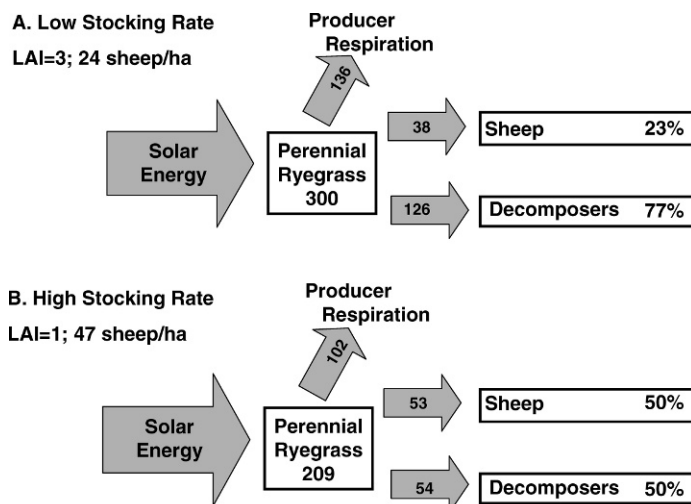
Figure 2. Illustration of the consequences of (A) low and (B) high stocking rate on energy partitioning ( \text{kg C}\cdot\text{ha}^{-1}\cdot\text{d}^{-1} ) between plant production and forage utilization by livestock in grazed ecosystems. Leaf area index (LAI) and forage utilization are interrelated so that neither can be optimized independently; rather, both must be simultaneously optimized to sustain plant and animal production. This fundamental requirement to balance plant growth and forage consumption by livestock partially explains why grazing research has found stocking rate to affect plant and animal response variables to a greater extent than grazing system on rangelands (redrawn from Parsons et al. 1983).
