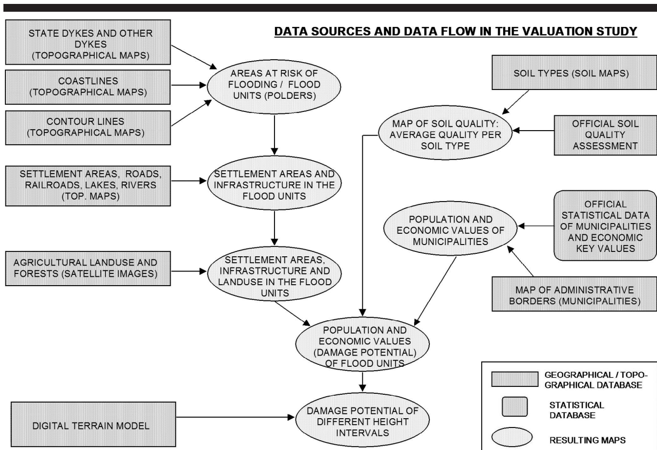
Figure 7. Data sources and step-wise GIS procedure in the meso-scale vulnerability study of the State of Schleswig-Holstein.
