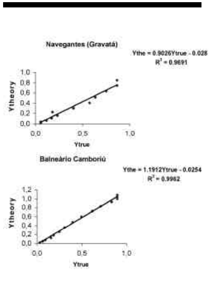
Figure 15. Relationship between Y_{theory} and Y_{true} for analysed features and the respective R^2 for salencies in Navegantes and Balneário Camboriú.
