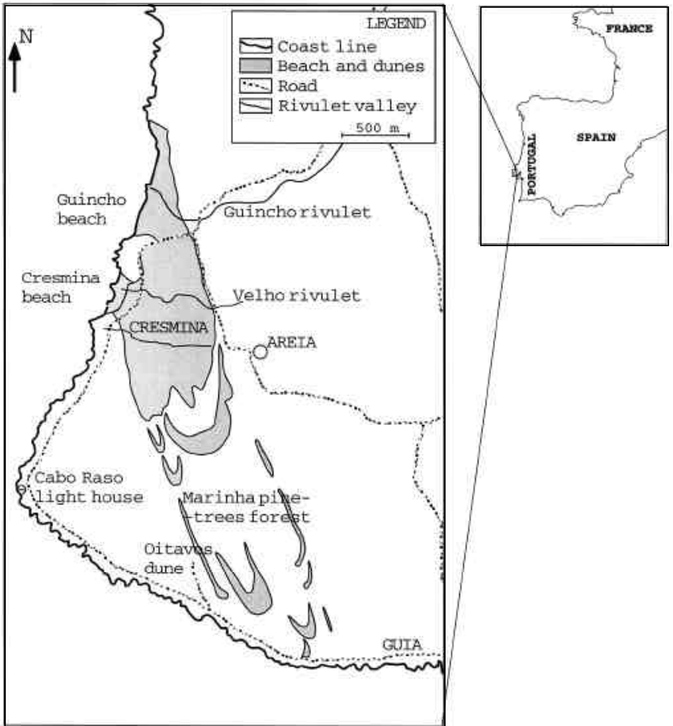
Figure 1. Guincho-Oitavos headland bypass dunefield localization and dune distribution.
