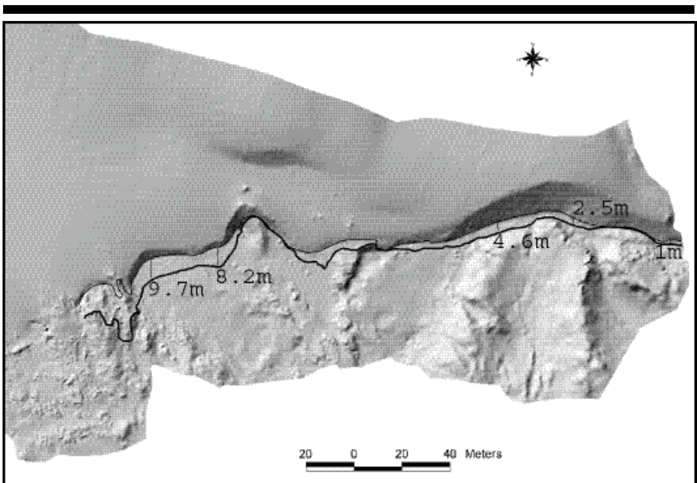
Figure 11. Cresmina's dune precipitation ridge advance from February 2000 to April 2001. Black lines represent the precipitation ridge position: Thick line, 2001 position and thin line the 2000. Values indicate the dune advance. 2000 DEM is shown as background.
