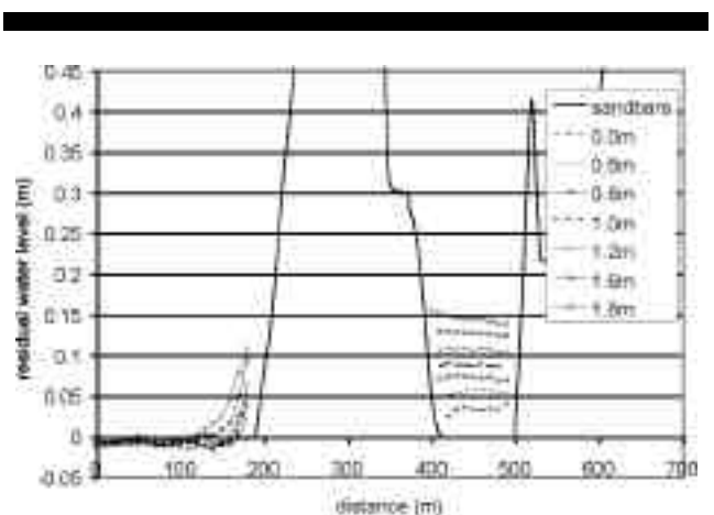
Figure 10. Wave condition effects along the Profile 3 ( P_3 = 0 m; P_3' = 700 m).
