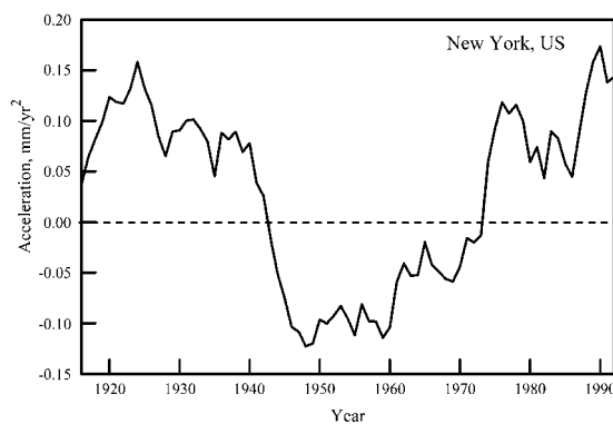
Figure 5. Sea-level acceleration at New York based on 46-year records centered in years 1916–1992 and representing the years 1893–2014.
