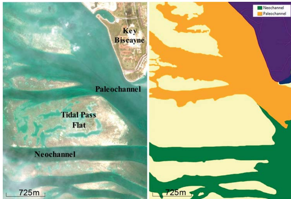
Figure 11. Detailed example of Channel Geoform interpretations using IKONOS-2 satellite imagery. The left panel shows the identification of associated landforms, which include Neochannel and Paleochannel, while the right panel overlays mapping units of specific color ( viz. Figure 4) on top of the satellite imagery to visually demonstrate spatial dynamics. In addition to the colors and units provided in the legend above, yellow areas in the right panel represent the Planar Bed Forms and Ripples Landform, which is a subclassification unit of the Sediment Flat Geoform; dark purple areas represent Karst Island Landforms; and dark blue areas represent Subtidal Pavement Landforms. A nominal scale of 1:16,000 was used for both panels when exported out of ArcMap.
