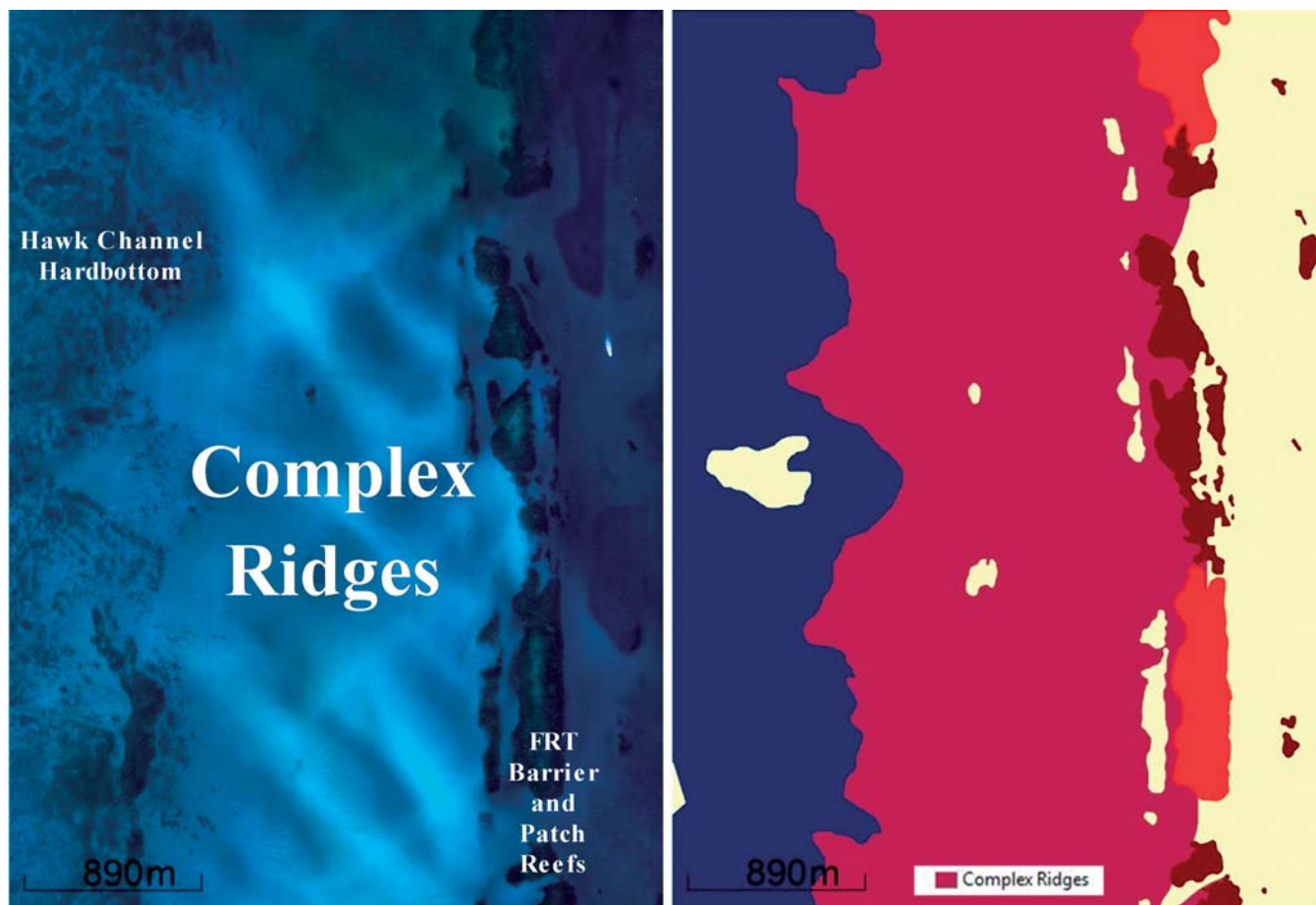
Figure 10. Detailed example showing distinctive spectral reflectance patterns for landforms associated with Coral Reef, Sediment Flat, Hardbottom, and Ridge Field Geofoms. The largest benthic feature identified in the left panel is the Complex Ridge Landform, which is located between the Hardbottom Geofoms of Hawk Channel and the Barrier and Patch Reef Landforms of the Florida Reef Tract (FRT). Notice how the high-resolution of the IKONOS-2 imagery is able to capture the characteristic crisscrossing pattern along the seafloor. The right panel overlays color-assigned classification units on top of the satellite imagery to visually demonstrate the distribution of landforms along the benthos. In addition to Complex Ridges, yellow areas in the right panel represent the Planar Bed Forms and Ripples Landform, which is a subclassification unit of the Sediment Flat Geofom; dark blue areas represent Subtidal Pavement Landforms; dark red areas represent Patch Reef Landforms; and bright red areas represent Barrier Reef Landforms. Both panels were exported out of ArcMap at a nominal scale of 1:19,000 within the layout view feature.
