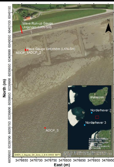
Figure 2. Measurement chain for nearshore waves, currents and hydrodynamic loads on the sea dike near Untjehörn, Island of Pellworm.
