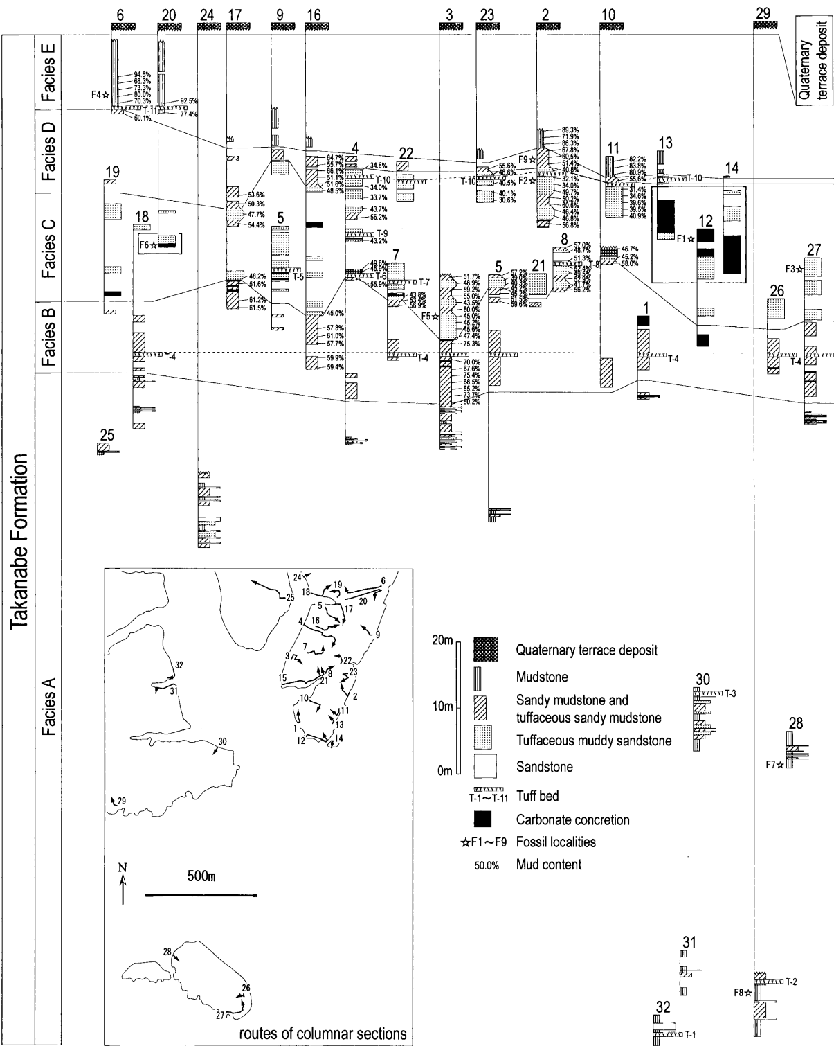
Figure 2. Stratigraphic sections of the upper Takanabe Formation in the study area. Facies A–E are described in the text. The rectangles indicate where the cold-seep assemblages occur: fossil localities F1 (Figure 5) and F6. The thicknesses of the tuff beds are not to scale, but are given in Table 1.
