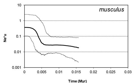
Fig. 8. Demographic history of M. m. domesticus , M. m. castaneus , and M. m. musculus population depicted as N_e * \mu (effective population size*mutation rate) plotted against time (in million years) as estimated with the Bayesian skyline plot model. The thick middle line is the median estimate whereas the thin line indicates upper and lower limits of 95 % highest posterior density (HPD).
