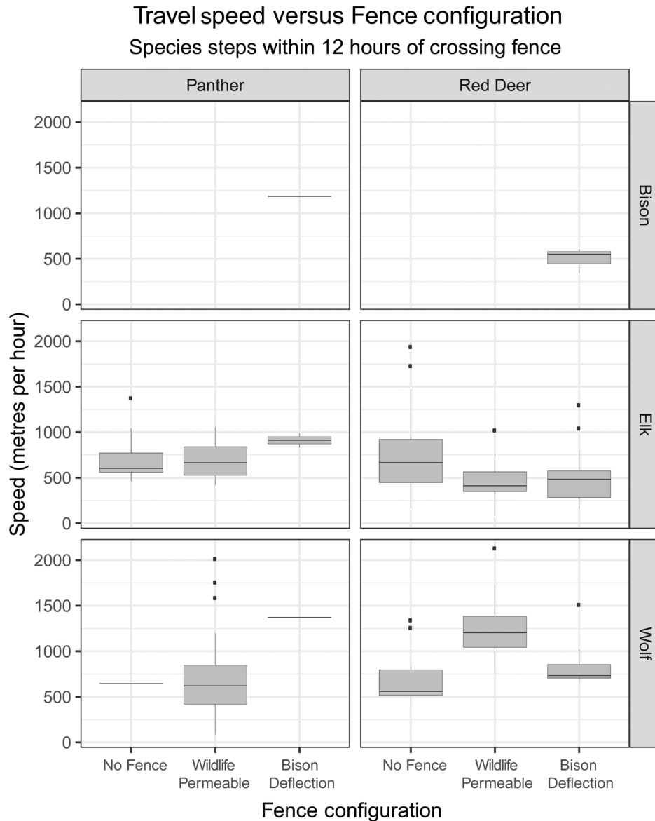
Figure 5. Boxplot of wildlife movement rates before and after two drift fence installations in separate valleys in Banff National Park. Average travel speed ( \text{m h}^{-1} ) derived from GPS telemetry steps within 12 h of animals approaching and departing fences in wildlife-permeable and bison-deflection configurations. No before or wildlife-permeable data for bison since they were not on the landscape prior to fence construction and only interacted with fences in bison-deflection configuration.
