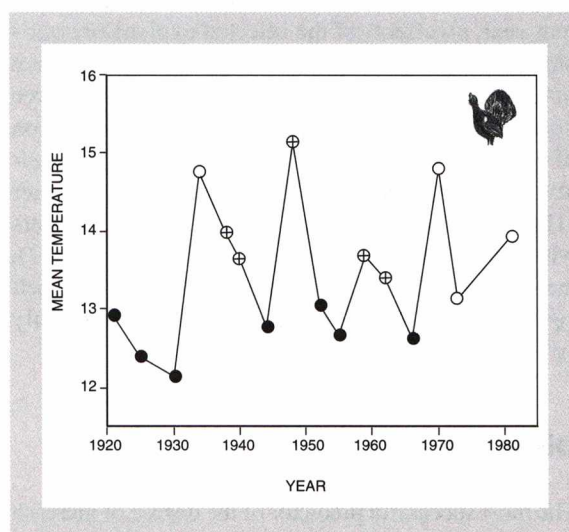
Figure 3. Mean temperature in June-September of the previous year for years with a bilberry production index below medium but a production above average in the previous year (1/0 years). The years were further categorised based on the autumn population size of capercaillie, compared to the size in the previous year. ● symbolises years with a strong increase, ⊗ years with a slight increase, and ○ years with no increase in the capercaillie autumn population.
