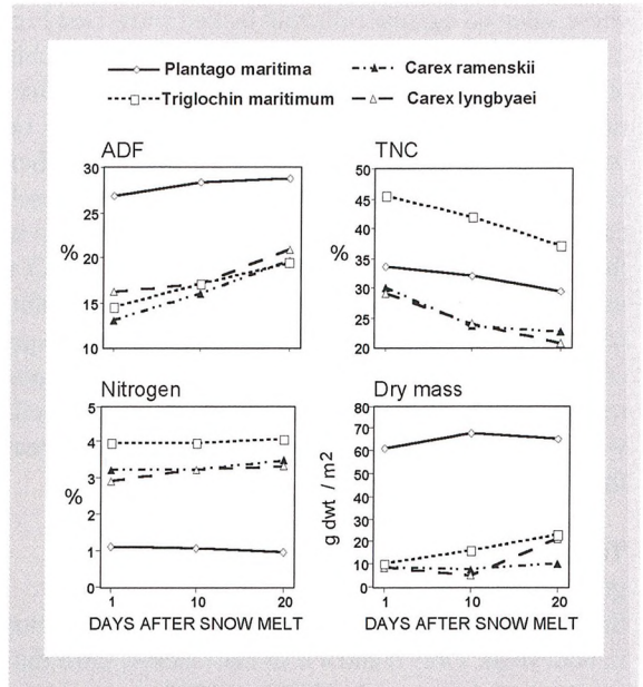
Figure 6. Change in biomass (g dry mass/m 2 ) and acid detergent fiber (ADF), total non-structural carbohydrate (TNC) and nitrogen concentrations (% dry mass) of major snow goose forage species following snow melt in Upper Cook Inlet, Alaska. Analysis was based on roots of Plantago maritima , shoots and rhizomes of Carex ramenskii , and shoots of Triglochin maritimum and Carex lyngbyaei , collected at four exclosed sites for each species, and three times following snow melt. Biomass and concentrations of ADF and nitrogen were averaged across sites, whereas sites were pooled to estimate TNC.
