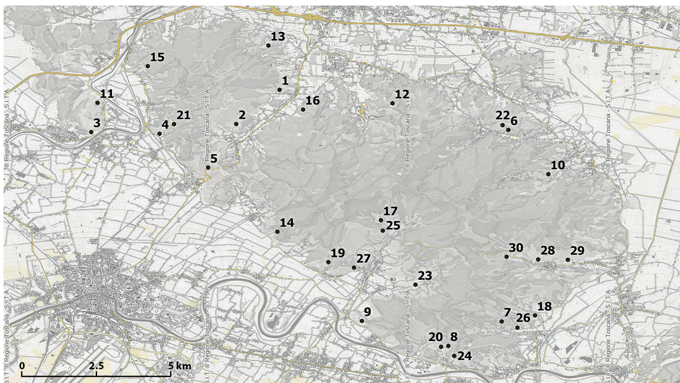
Fig. 1: Map of the sites sampled in 2010 (6), 2013 (12) and 2014 (18) in the Monte Pisano area. The city of Pisa is in the lower left of the map. Detailed information (coordinates, altitude, year and microhabitats) for each site is reported in Tab.1.
