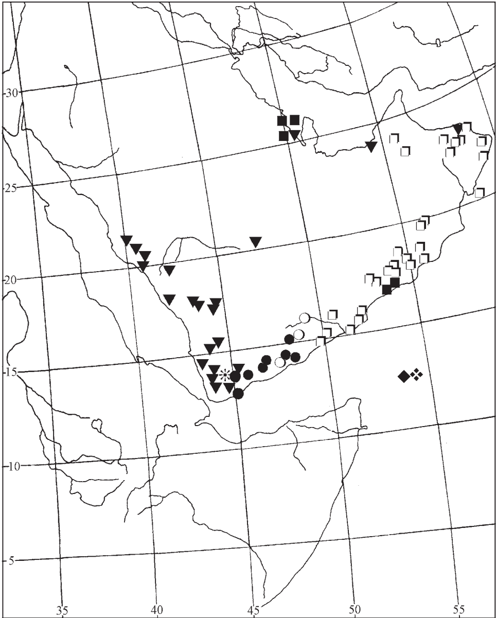
Fig. 1. Distribution of Pluchea arabica (□), P. dioscoridis (▼), P. glutinosa (◆), P. indica subsp. indica (○), P. indica subsp. yemenensis (●), P. ovalis (■), P. sordida (*).
