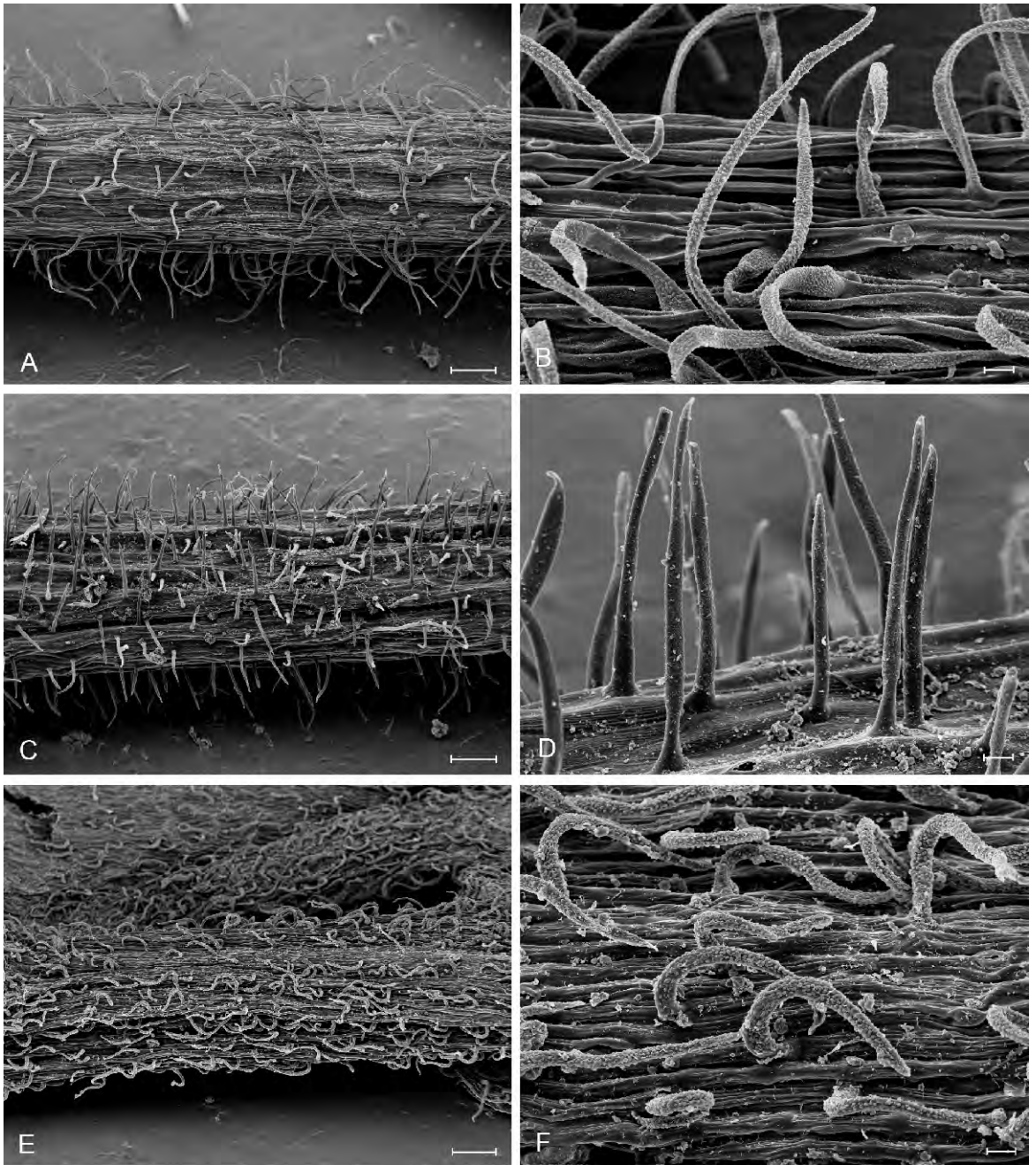
Fig. 4. SEM micrographs of the indumentum of Polygala rausiana (A, B) and related species (C-F) – A-B: P. rausiana ; C-D: P. peshmenii ; E-F: P. pruinosa subsp. pruinosa . – Material: P. rausiana (type locality, 29.5.2007, Raabe s.n., B); P. peshmenii (Eren 36/06, B); P. pruinosa subsp. pruinosa (Turkey, Yumru Dağı, 3.7.1992, Parolly s.n., B). – Scale bars: A, C, E = 200 \mu m, B, D, F = 20 \mu m.
