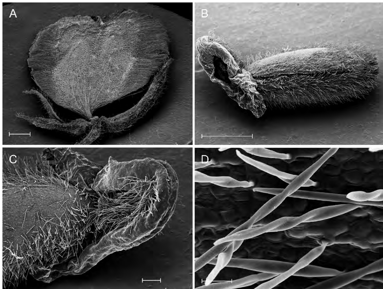
Fig. 3. SEM micrographs of Polygala rausiana – A: capsule, B: seed, C: strophiole, D: detail of the trichomes of the seed indumentum. – Material: Evrostina, 20.5.2007, Raabe s.n. (B). – Scale bars: A-B = 1 mm, C = 200 \mu m, D = 20 \mu m.
