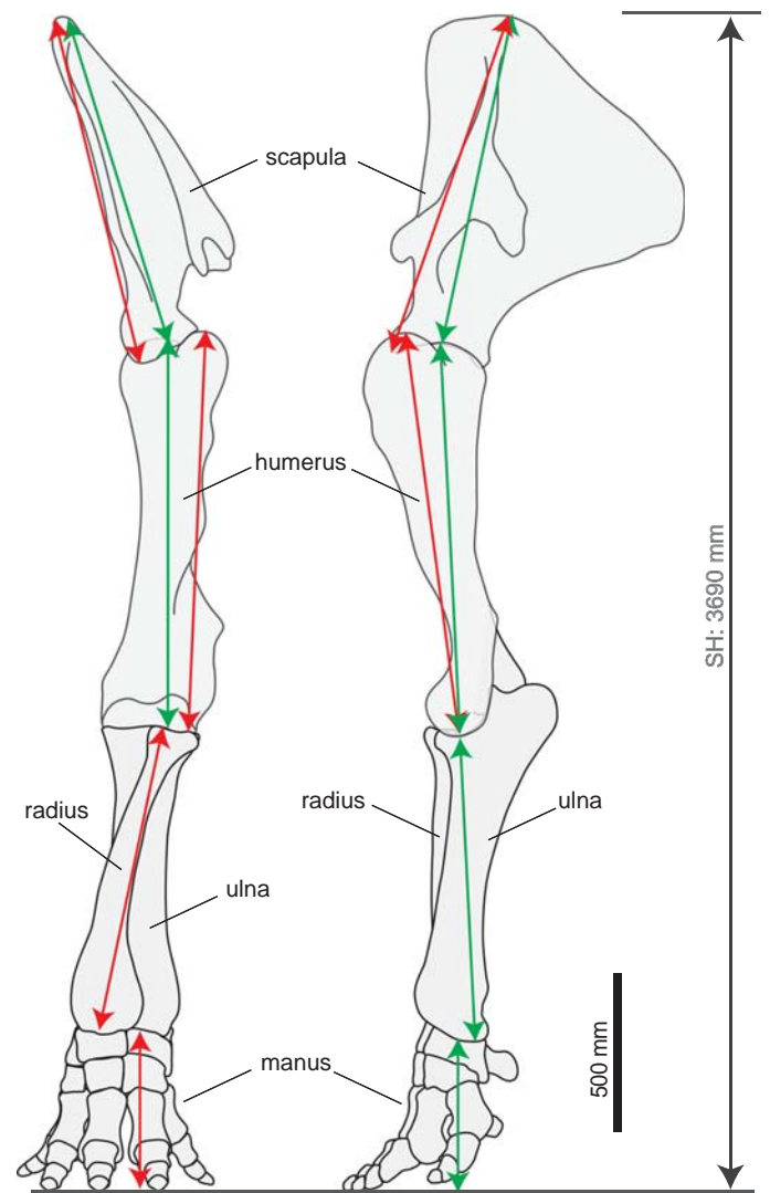
Fig. 1. Reconstruction of the forelimb of the Zhalainuoer III mammoth in anatomical position. The actual shoulder height (black): total height in anatomical position 3690 mm. The height obtained by adding the articular (green): manus (500 mm) + ulna (960 mm) + humerus (1233 mm) + scapula (1075 mm) = 3768 mm. Maximal lengths of different bone elements (red): manus (500 mm) + radius (985 mm) + humerus (1274 mm) + scapula (1115 mm) = 3874 mm. The actual shoulder height can be calculated by multiplying the result by 0.98 in the case of the sum of articular lengths and by 0.95 in the case of maximal lengths.
