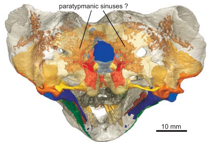
Fig. 3. Distribution of cavities in the otic region of the non-mammalian synapsid Pristerodon mackayi Huxley, 1868 (MB.R.985) from the Late Permian of Biesjespoort, South Africa. Note the concentration of a number of large cavities (brown) around the inner ears, which are connected to each other. The neurocranium is shown transparent.
