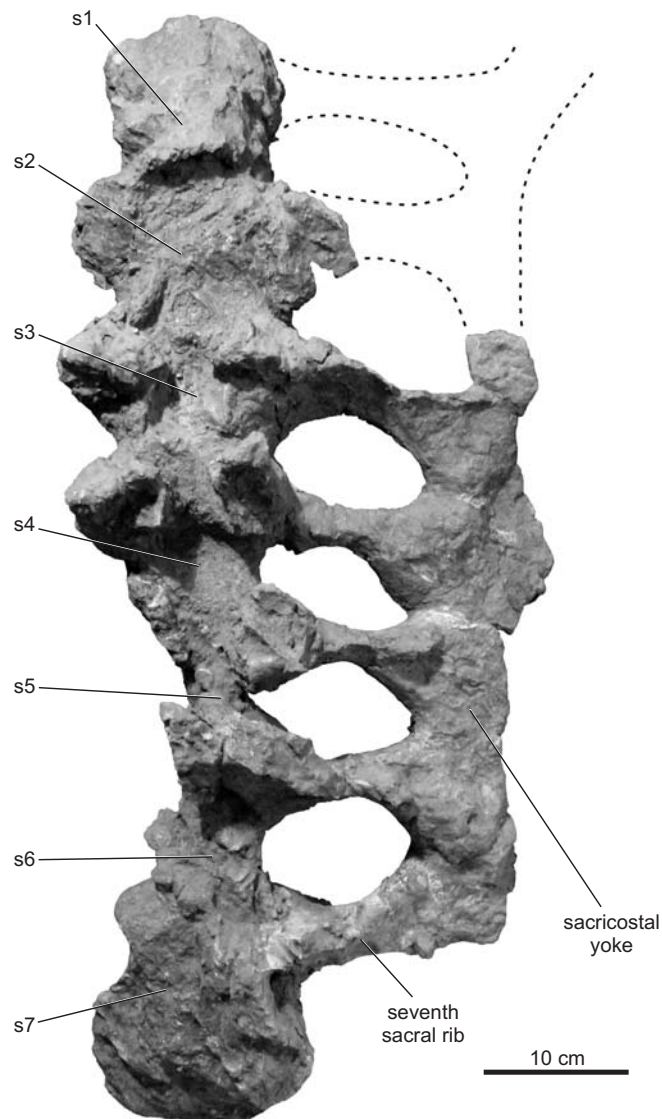
Fig. 7. Sauropod sacrum PVL 4017-18 from the Saltasaurus loricatus Bonaparte and Powell, 1980 quarry at El Brete, Argentina in dorsal view. Note the presence of seven sacral vertebrae. The abbreviations (s1–s7) indicate sacral vertebral identity. Dashed lines indicate missing bone.
