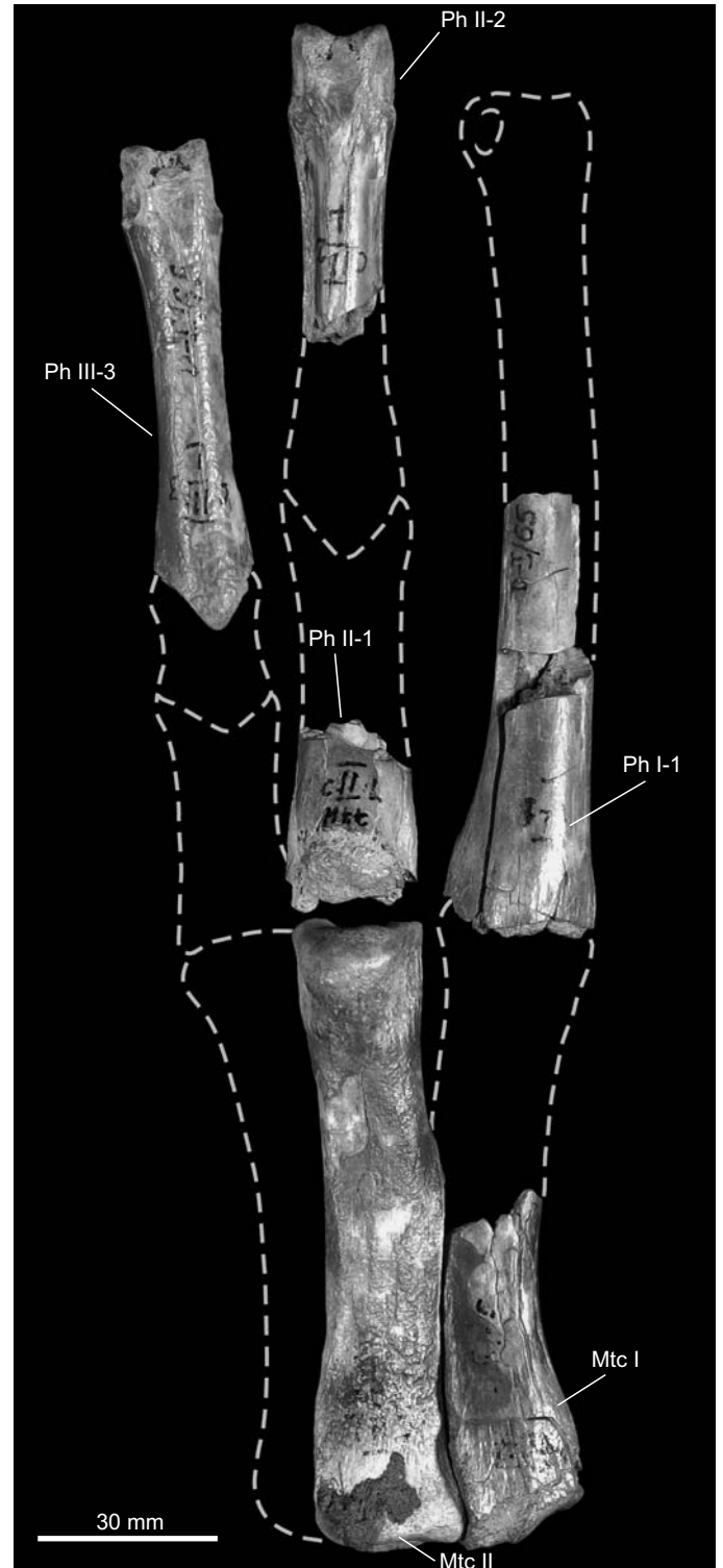
Fig. 4. Left manual bones of the ornithomimid ZPAL MgD-I/65 from the Upper Cretaceous Nemegt Formation, Mongolia shown without unguals, in dorsal view. Dashed lines indicate missing bones. Abbreviations: Mtc, metacarpal; Ph, phalanx.
