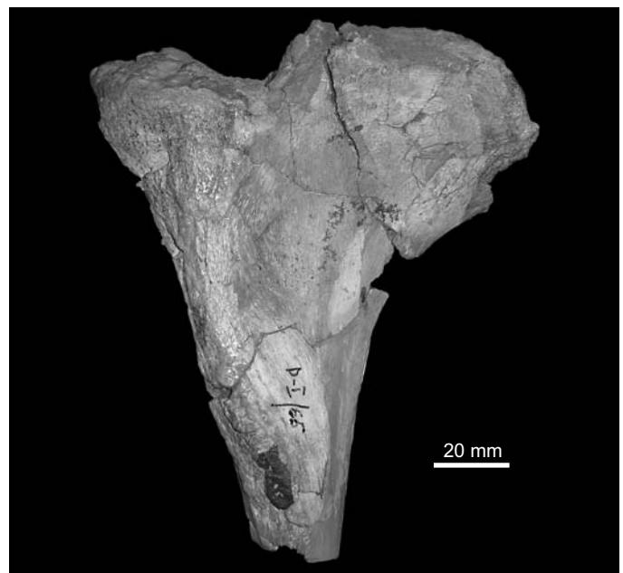
Fig. 6. Proximal part of the left pubis of the ornithomimid ZPAL MgD-I/65 from the Upper Cretaceous Nemegt Formation, Mongolia shown in lateral view.
