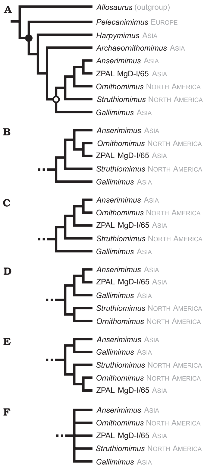
Fig. 11. Results of the phylogenetic analysis performed with PAUP 4.0 Beta 10 and PAST. Solid circle indicates Ornithomimosauria, open circle indicates Ornithomimidae. The tree A shows the full results of the phylogenetic analyses with outgroup taxon and non-ornithomimid ornithomimosaurians plus Ornithomimidae. Topologies of all trees to the level of Archaeornithomimus are identical hence the remaining trees ( B , C , D , E , F ) show only the relationships within Ornithomimidae. The tree F shows the strict consensus tree. To the right of each ornithomimosaurian taxon its geographical provenance has been given.
