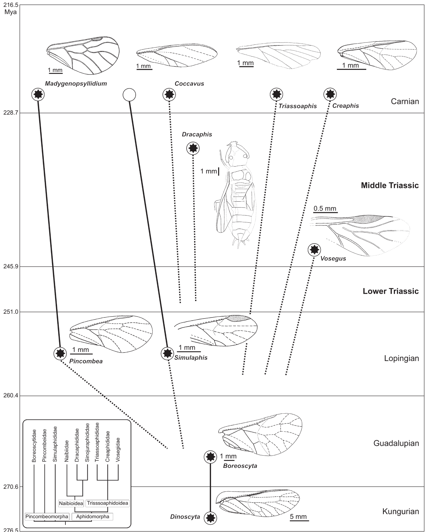
Fig. 3. Schema of range and relationships of Permian and Triassic Aphidomorpha and their relatives. Asterisks in circle, mean taxa figured in the schema; empty circle, non figured taxon. Inset: supposed cladogram of Permian and Triassic Aphidomorpha, inferred from data and opinions from Shcherbakov (2007) and Heie and Wegierek (2009a, b).
