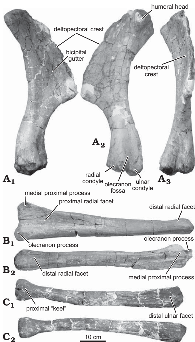
Fig. 19. Hadrosaurid dinosaur Olorotitan arharensis Godefroit, Bolotsky, and Alifanov, 2003 (AEHM 2/845, holotype), from the Upper Cretaceous of Kundur (Russia). A. Left humerus, in cranial ( A_1 ), caudal ( A_2 ), and lateral ( A_3 ) views. B. Right ulna, in cranial ( B_1 ) and medial ( B_2 ) views. C. Right radius, in caudal ( C_1 ) and cranial ( C_2 ) views.
