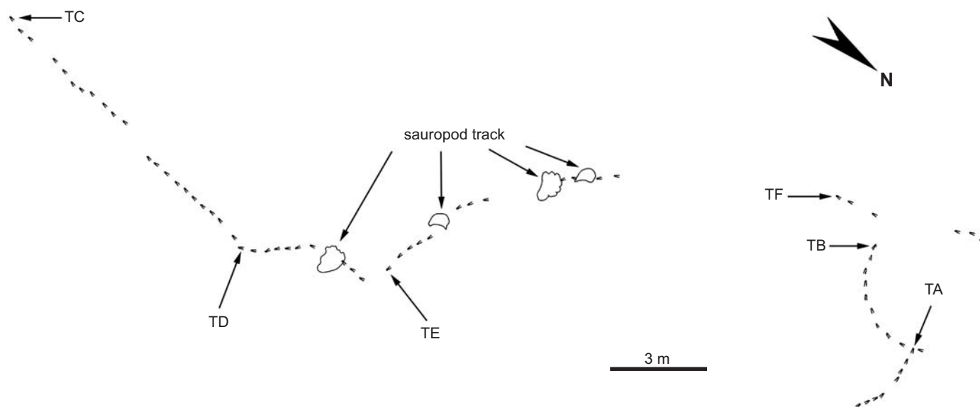
Fig. 5. Schematic map of the relative positions of six Dromaeosauripus yongjingensis trackways (GSLTZP-S2-TA to TF) at Liujiaxia Dinosaur National Geopark site II, Early Cretaceous.
