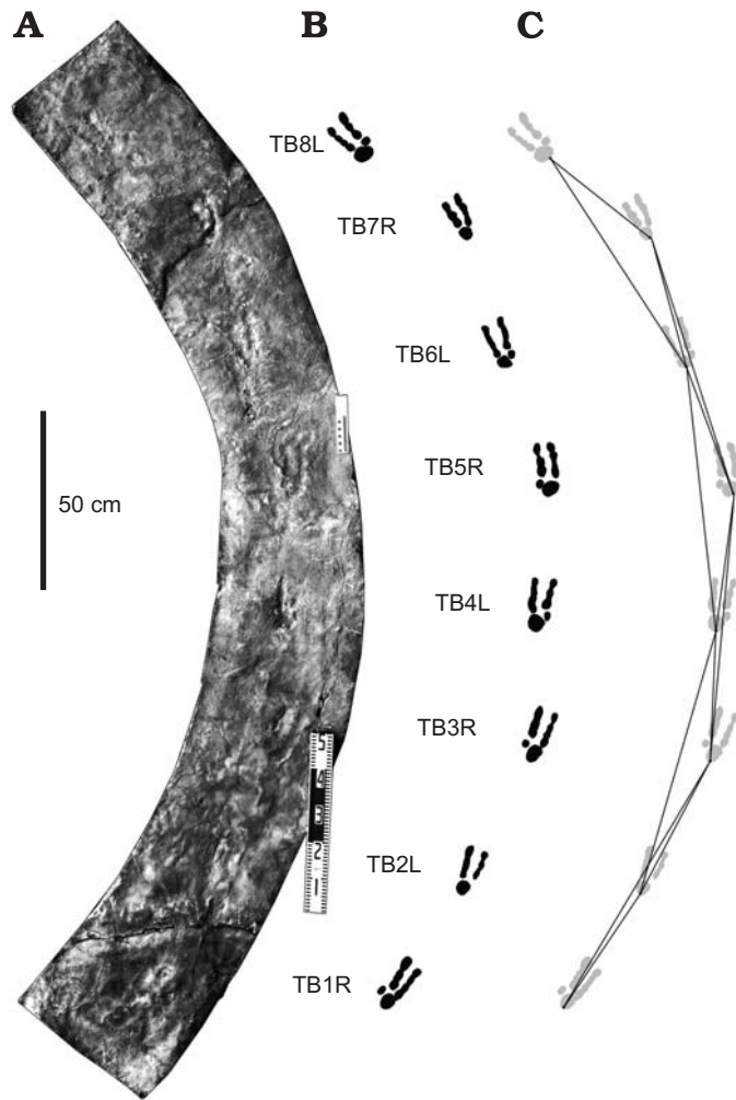
Fig. 4. Turning trackway of Dromaeosauripes yongjingensis GSLTZP-S2-TB at Liujiaxia Dinosaur National Geopark site II, Early Cretaceous. A. Photograph. B. Outline drawing. C. Pace angulations.
