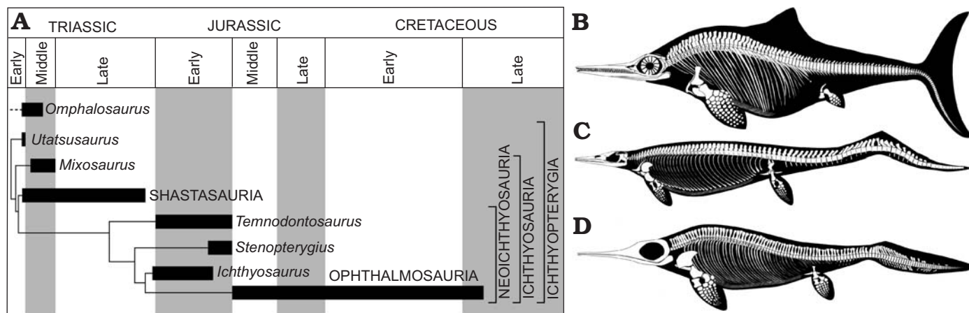
Fig. 1. Simplified view of the evolution of the Ichthyopterygia. A . Time-calibrated phylogenetic tree of the Ichthyopterygia. B–D . Schematic drawings (from McGowan and Motani 2003) showing the evolution of the body plan within the Ichthyopterygia (not to scale), between the basal ichthyopterygian Utatusaurus ( B ), the basal ichthyosaurian Mixosaurus ( C ), and the scombrid fish-shaped neoichthyosaurian Ophthalmosaurus ( D ). Stratigraphic data compiled after McGowan and Motani (2003), Fernández (2003), Bennett et al. (2012), and Wiman (1910).
