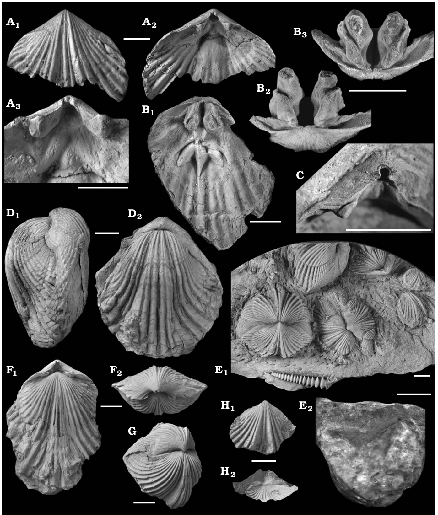
Fig. 14. Trigonorhynchiid brachiopod Plectothyrella crassicosis (Dalman, 1828) from the Kuldiga Formation of the Porkuni Regional Stage, Hirnantian (Upper Ordovician), East Baltic, western Latvia. A. Ventral valve, LDM G 328-15, Blīdene-5, depth 816.6 m, exterior view (A 1 ), interior view (A 2 ) and the detail of the posterior part of the same (A 3 ). B. Incomplete dorsal valve, GIT 542-16, Riekstini-15, 854.8 m, dorsal interior (B 1 ), posterior (B 2 ), and posteriorly tilted (B 3 ) views of cruralium. C. Ventral valve, LDM G 328-149, Mežmali-16, depth 914.9 m, view of pedicle opening. D. Shell, LDM G 328-135, Ēdole-61, 848.1 m, lateral (D 1 ) and dorsal (D 2 ) views. E. Shells, GIT 542-3/1-3, Adze-6, 838.5 m, posterior views of shells in live position and →
