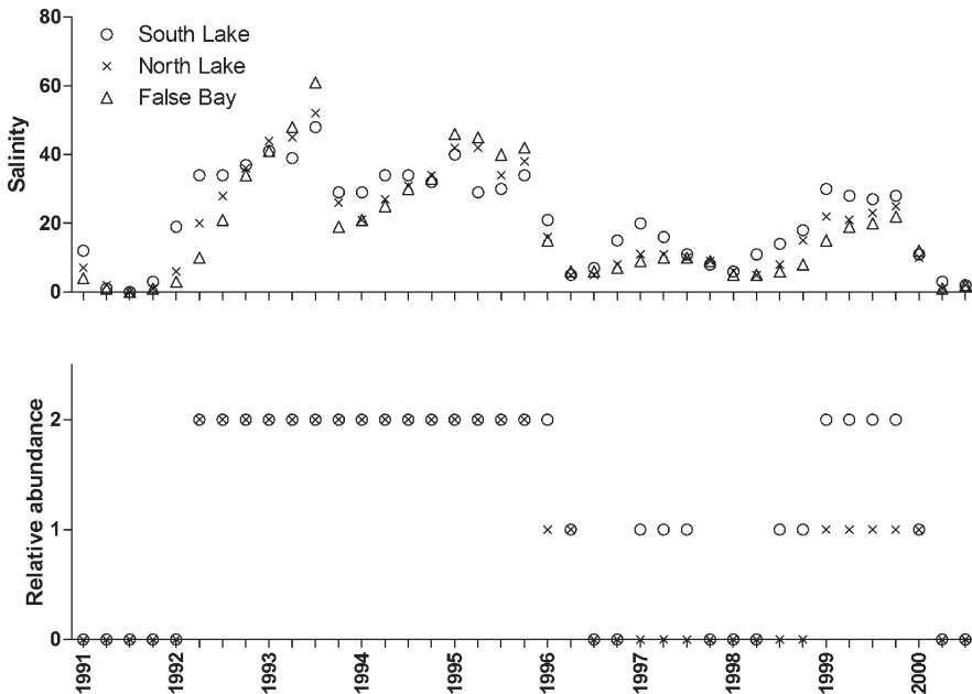
Fig. 3. Salinity and relative abundance of Crambionella stuhlmanni recorded in the St Lucia Estuary from 1991 to 2000. Abundance: 0 – absent, 1 – present, 2 – abundant.
