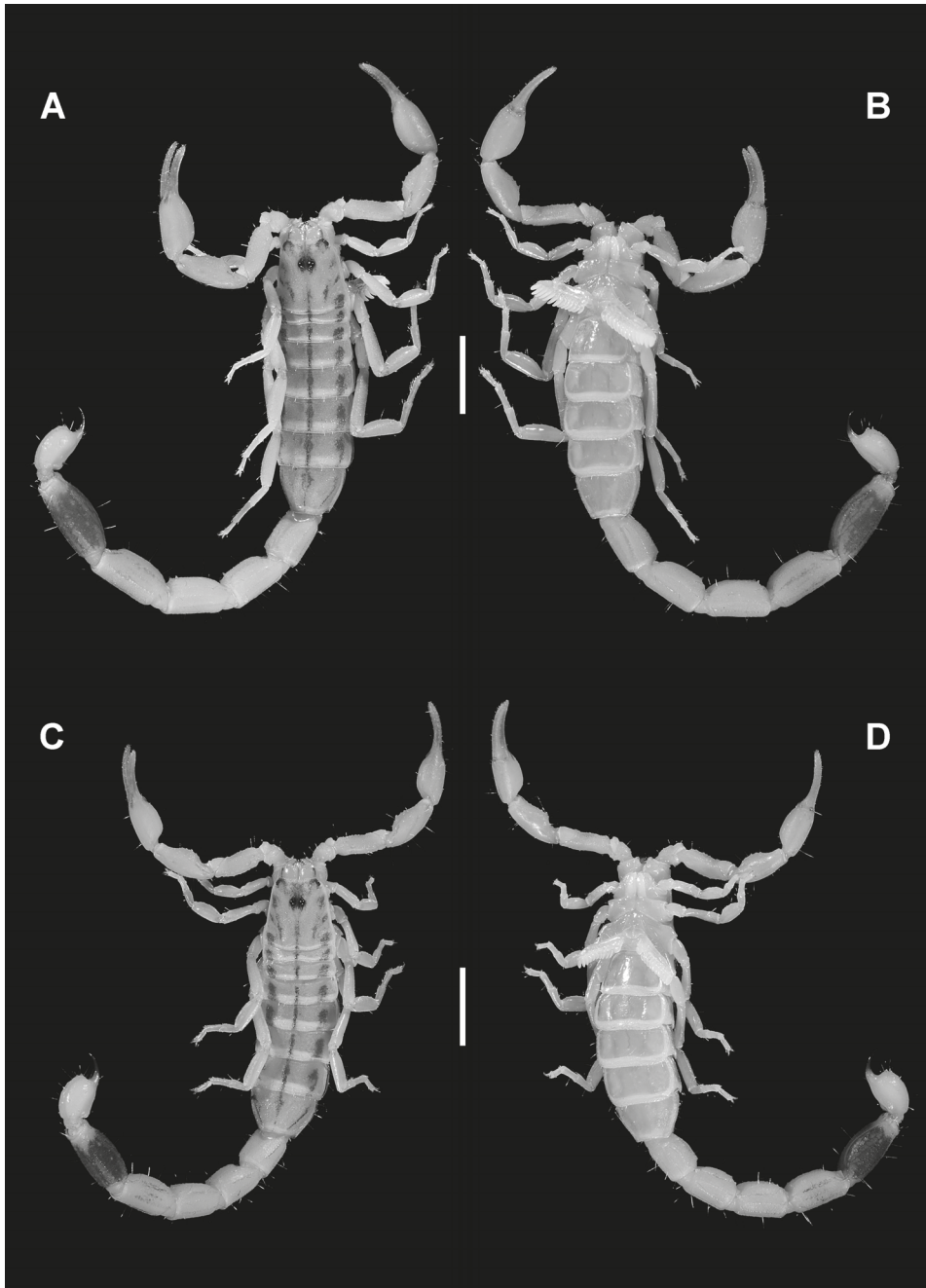
Fig. 4. Habitus, (A, C) dorsal aspect and (B, D) ventral aspect of Uroplectes ansiedippenarae sp. n., Loeriesfontein, Northern Cape Province, South Africa. A, B – Holotype ♂ (AMNH); C, D – Paratype ♀ (AMNH). Scale bars = 5 mm.
