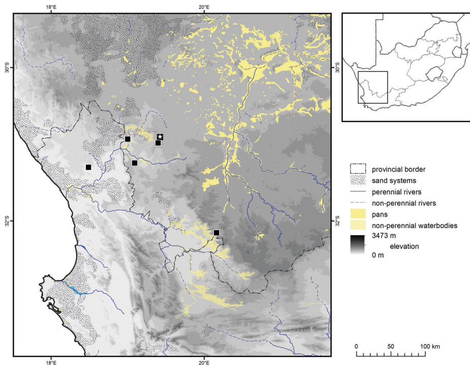
Fig. 1. The known distribution of Uroplectes ansiedippenarae sp. n. in the Northern Cape and Western Cape provinces of South Africa. Black squares indicate known locality records; white star on black square indicates type locality.
