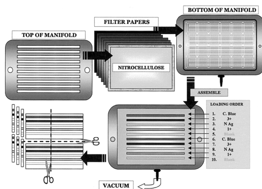
FIGURE 1. Protocol for the manufacture of strip immunoblot assays (SIA). We sandwiched a pre-sized nitrocellulose membrane between the lower (vacuum) and upper panels of an Immune SB-10 mini slotter, and then applied Coomassie brilliant blue (C. Blue), diluted deer mouse serum (3+ and 1+), and recombinant nucleocapsid antigen (N Ag) in separate wells in a total volume of 1 ml each. After applying the vacuum, we removed the membrane and cut it lengthwise with a paper shredder to produce the SIA strips.
