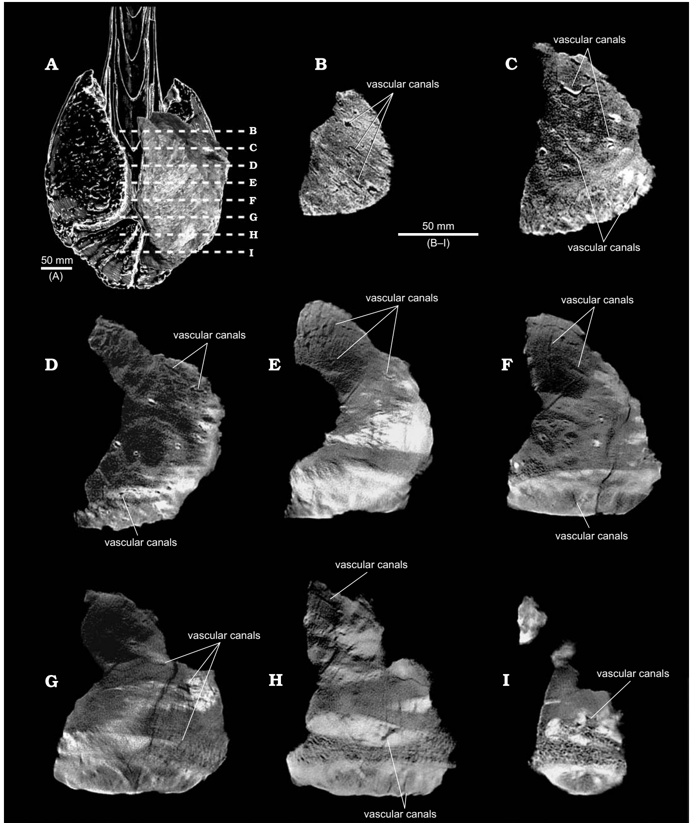
Fig. 9. A tail club from an indeterminate ankylosaurid (probably Euoplocephalus ), TMP 2000.57.03, from the Upper Cretaceous Dinosaur Park Formation of Alberta. A . External surface photograph of specimen. The sketch in panel A is from Carpenter (2004). B–I . CT images of a terminal osteoderm of the tail club of an indeterminate ankylosaurid (TMP 2000.57.03) from the Upper Cretaceous Dinosaur Park Formation of Alberta; see also Fig. 7. The tail club has a complex vascular network. Dashed lines in A indicate cutting planes.
