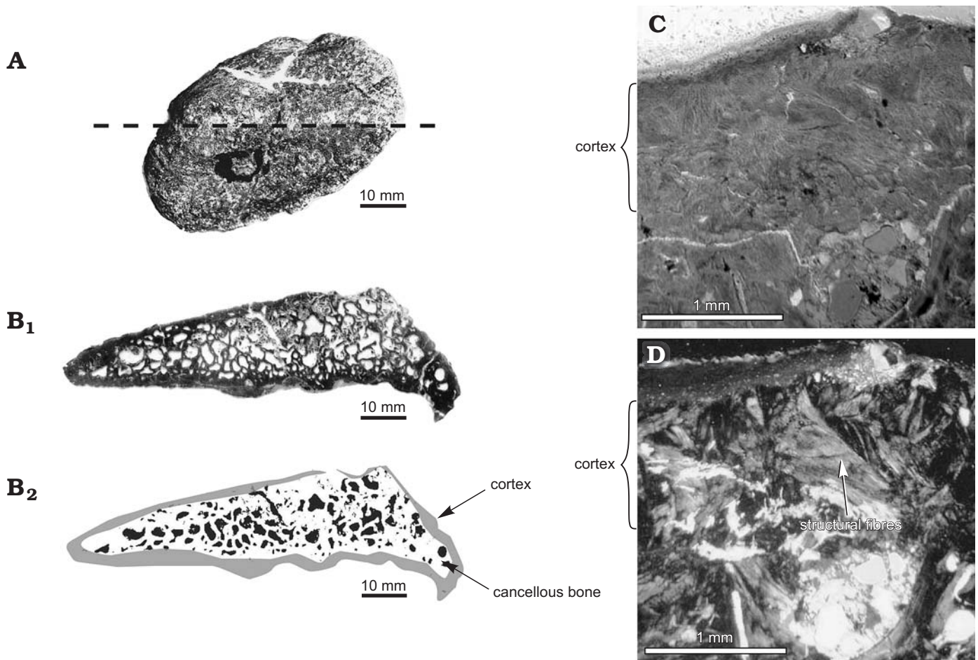
Fig. 3. An osteoderm from the polacanthid Gargoyleosaurus parkpini (DMNH 27726) from the Upper Jurassic Morrison Formation of Utah. A . Photograph of the external surface of the specimen. B . Thin-section of an osteoderm, cut along indicated by dashed line in A . The thin-section was cut parallel to the ridge of the osteoderm; photograph ( B 1 ) and interpretive drawing ( B 2 ). The cortex in the section completely surrounds the inner cancellous bone; dark gray, cortical bone consisting of woven or structural fiber bone; white, cancellous bone. C , D . Cortical bone tissue of the osteoderm. Detail of the cortex and inner trabecular bone in normal ( C ) and polarized ( D ) light; external surface is to the top. Many structural fiber bundles occur within the cortex.
