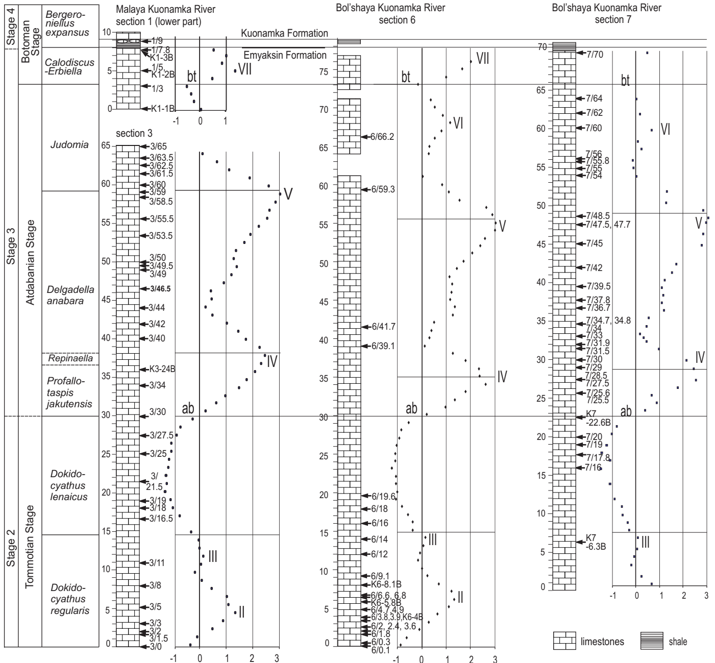
Fig. 2. Derivation of fossiliferous samples (arrows with numbers) and chemostratigraphic correlation of sections 1 and 3 (Malaya Kuonamka River) with sections 6 and 7 (Bol'shaya Kuonamka River). Correlation with carbon isotope features II–VII from stratotypes of south-eastern Siberian Platform (Brasier et al. 1994) according to Kouchinsky et al. (2001). Note that the zero level in all sections corresponds to the water level above which the sections were exposed in 1996. Description of fauna from the lower part of the Emyaksin Formation in complementary outcrops at the Bol'shaya Kuonamka River (below that zero level) will be published elsewhere. Fauna from the overlying Kuonamka Formation is published by Gubanov et al. (2004) and Kouchinsky et al. (2011).
