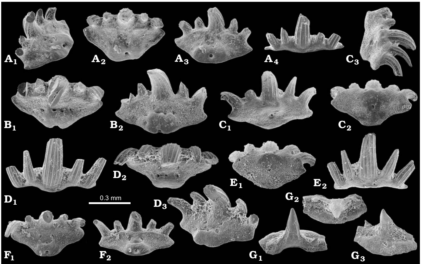
Fig. 7. Cladodont teeth from the upper Viséan of Cawdor Quarry, Matlock, Derbyshire, England, UK; sample Cawdor 9 (A–C), 11 (D–G). A–F. Denaëa cf.ournieri Pruvost, 1922. A. NHMUK PV P73276, in lateral (A 1 ), oral (A 2 ), lingual (A 3 ), and labial (A 4 ) views. B. NHMUK PV P73277, in oral (B 1 ) and lingual (B 2 ) views. C. NHMUK PV P73278, in aboral (C 1 ) and aboral/labial (C 2 ) views. D. NHMUK PV P73279, in labial (D 1 ), oral (D 2 ), and oblique lingual (D 3 ) views. E. NHMUK PV P73280, in aboral (E 1 ) and labial (E 2 ) views. F. NHMUK PV P73281, in oral (F 1 ) and lingual (F 2 ) views. G. Squatinactis caudispinatus Lund and Zangerl, 1974, narrow tooth with broken base (NHMUK PV P73282), in labial (G 1 ), oral (G 2 ), and lingual (G 3 ) views.
