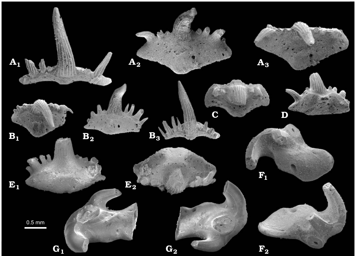
Fig. 10. Chondrichthyan teeth from the upper Viséan of the Westenfeld Quarry, Rhenish Mountains, Germany. A–E. Denaea cf. fournieri Pruvost, 1922. A. MWGUW/Ps/11/1, in labial (A 1 ), lingual (A 2 ), and oral (A 3 ) views. B. MWGUW/Ps/11/2, in oral (B 1 ), lingual (B 2 ), and labial (B 3 ) views. C. MWGUW/Ps/11/3, in oral view. D. MWGUW/Ps/11/4, in labial/aboral view. E. MWGUW/Ps/11/5, in lingual (E 1 ) and oral (E 2 ) views. F, G. Thrinacodus cf. gracia (Grogan and Lund, 2008). F. MWGUW/Ps/11/6, in oral (F 1 ) and lateral (F 2 ) views. G. MWGUW/Ps/11/7, in lateral (G 1 ) and oral (G 2 ) views.
