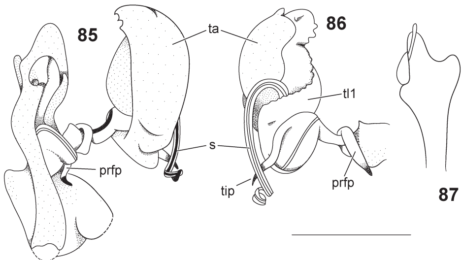
Figs 85–87. Spinotarsus xanthonotus Attems, ♂: (85) gonopod, aboral view; (86) telopodite, oral view; (87) telocoxite, oral view. Abbreviations: ( s ) solenomere, ( prfp ) prefemoral process, ( ta ) tarsal lobe, ( tip ) tibial process, ( tl1 ) basal lobe of tarsus. Scale bar = 1 mm.
