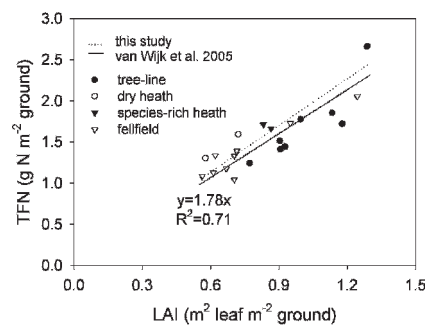
FIGURE 5. Relationship of total foliar nitrogen (TFN) vs. leaf area index (LAI) for different arctic communities dominated by Cassiope tetragona . The TFN-LAI relationship for generic arctic tundra (van Wijk et al., 2005) is also shown.
