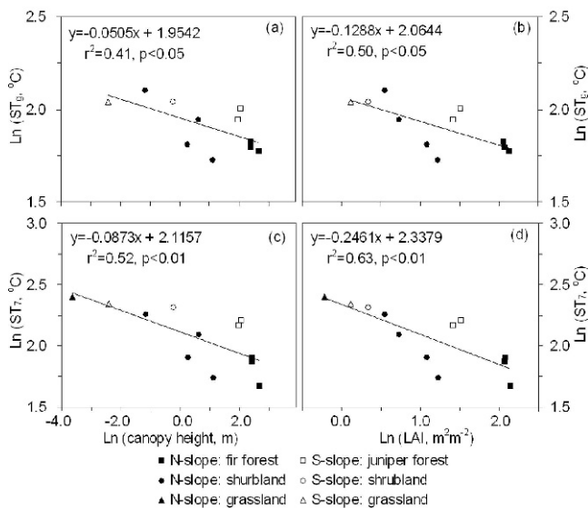
FIGURE 5. Relationships of mean soil temperatures for growing season ( ST_g ) and July ( ST_7 ) to (a, c) canopy height and (b, d) LAI across 12 plots with altitudinal vegetation changes from forests to shrublands and grasslands in the Sergyema Mountains. All variables were in natural logarithmic transformation (original data found in Tables 1 and 3). The trend lines were for the data pooled from the 12 plots.
