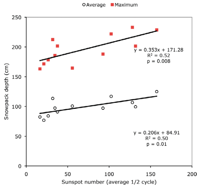
FIGURE 4. Relationship between snow cover in the Snowy Mountains of Australia and sunspot numbers for half a cycle (5–6 years).
