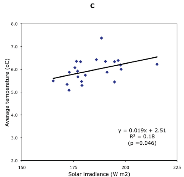
FIGURE 6. Annual average air temperature in the Snowy Mountains in relation to (A) atmospheric CO 2 concentrations; (B) the Southern Oscillation Index (SOI); and (C) surface solar irradiance.
