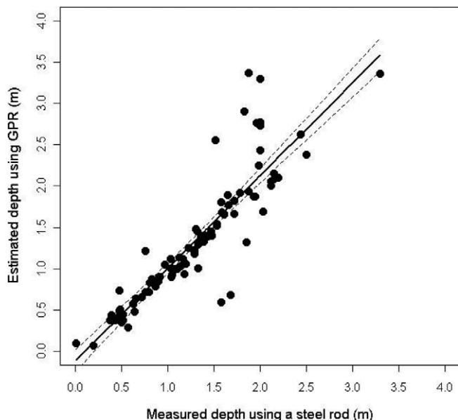
FIGURE 2. Ninety percent confidence intervals (dashed lines) of the linear regression (solid line) between direct measurements of snow depth and estimated values of depth obtained from GPR data.
