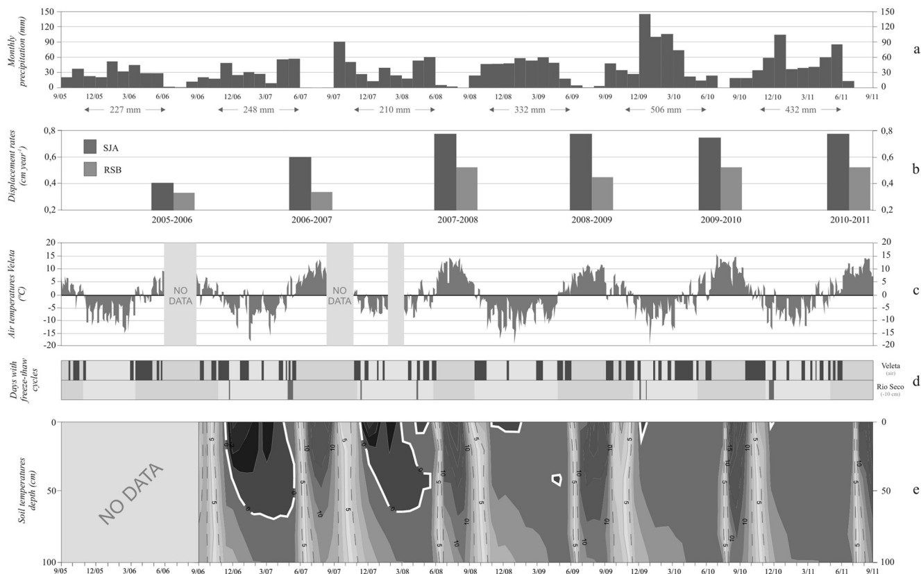
FIGURE 3. (a) Monthly precipitation at Granada weather station and total precipitation between November and June. (b) Mean annual horizontal movement rates at elevation belt SJA and solifluction area RSB. (c) Daily air temperatures at Veleta Peak. (d) Days with freeze-thaw cycles at Veleta Peak and at 10 cm depth in a solifluction lobe from the Rio Seco cirque. (e) Ground thermal conditions in the same solifluction lobe.
