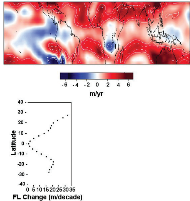
FIGURE 3. Changes in tropical freezing level heights for the period 1977–2007 (top panel) and profile of zonally averaged values (bottom panel). After Bradley et al. (2009).
