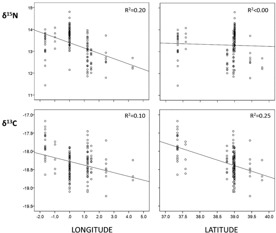
FIG. 3.— Relationship between \delta^{15}\text{N} and \delta^{13}\text{C} values in P1 feathers of European Storm-petrels and latitude and longitude of their respective breeding sites across the Western Mediterranean. Both relationships with \delta^{13}\text{C} , and longitude with \delta^{15}\text{N} , were significant.
