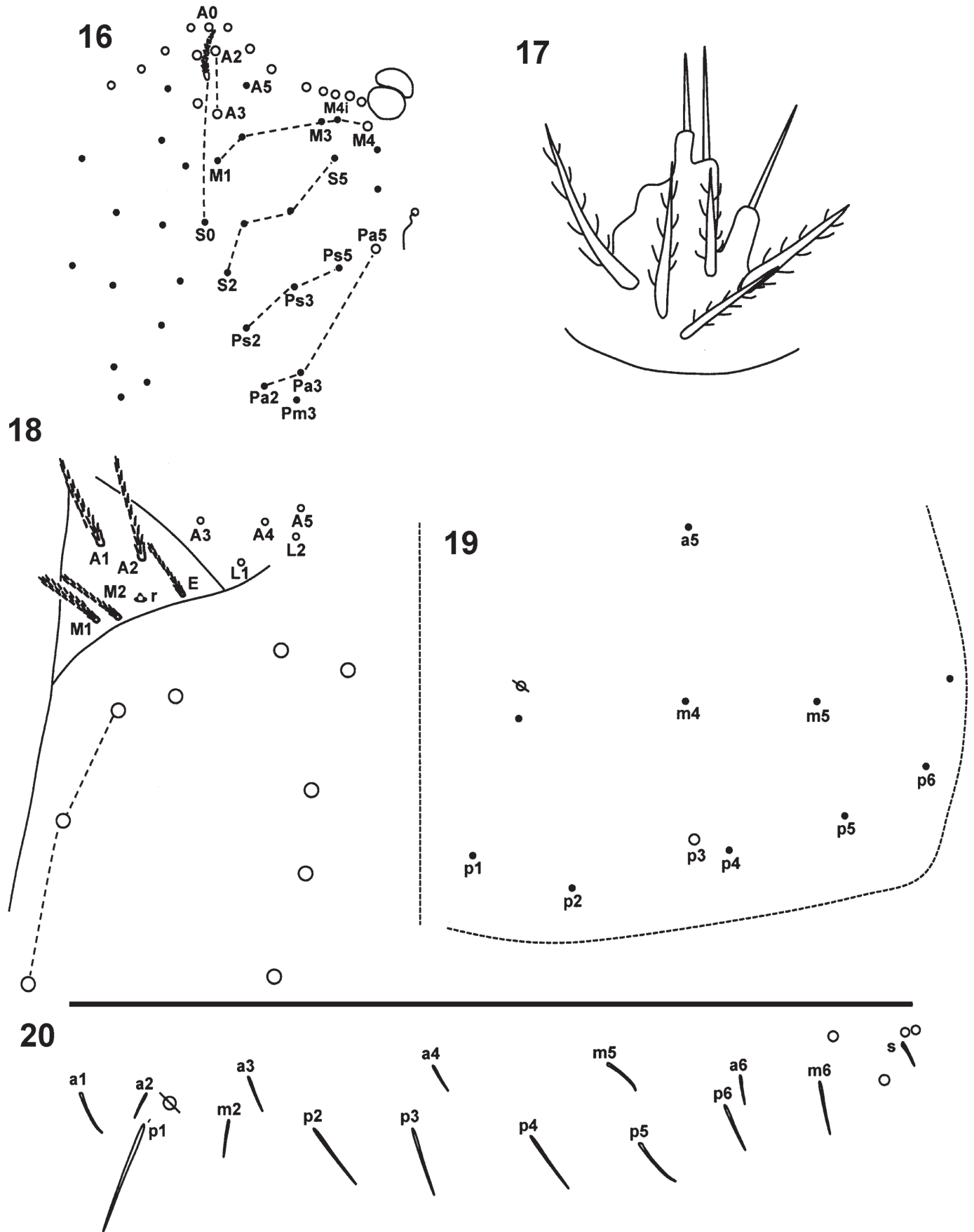
Figs. 16–20. Metasinella radkei sp. nov. (16) Dorsal chaetotaxy of head. (17) Proximal setae of labial palp. (18) Labial and postlabial setae, all elements are coarsely ciliate. (19) Mesothorax. (20) Metathorax.
