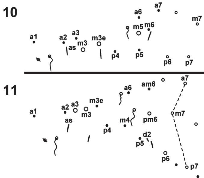
Figs. 10–11. Dicranocentrus icelosmaris sp. nov. dorsal chaetotaxy. (10) Second abdominal segment. (11) Third abdominal segment.
