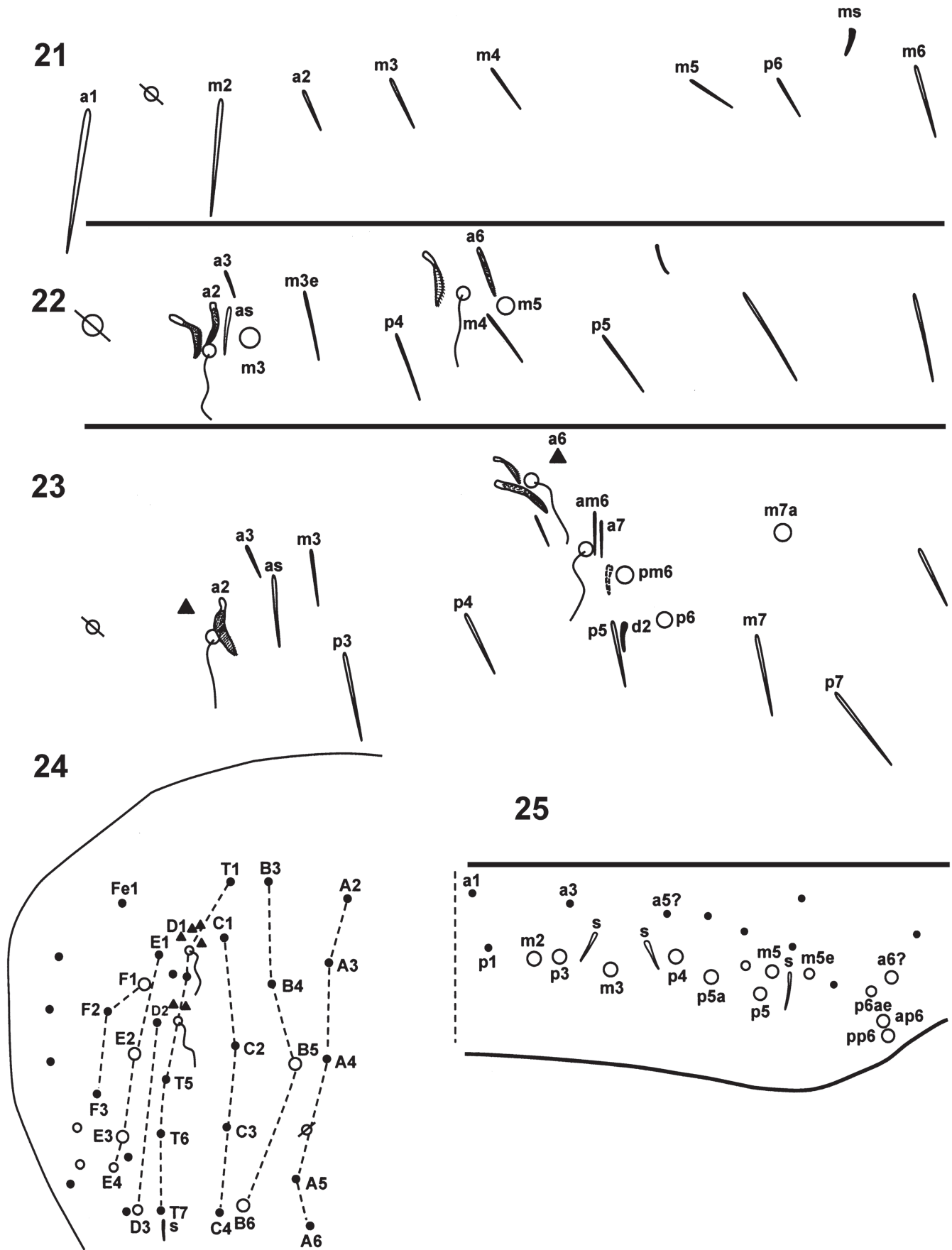
Figs. 21–25. Metasinella radkei sp. nov. Abdominal chaetotaxy on (21) 1st segment; (22) 2nd segment; (23) 3rd segment, hatched line shows alternative insertion of d2; (24) 4th segment; (25) 5th segment.
